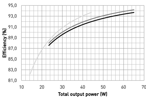
Typical efficiency
