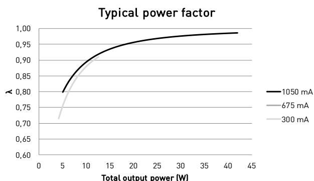
Current value is adjustable in steps via dip-switch. See dip-switch settings in page 3 for details.
