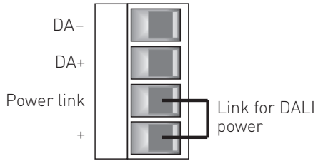
-- DALI supply connections
