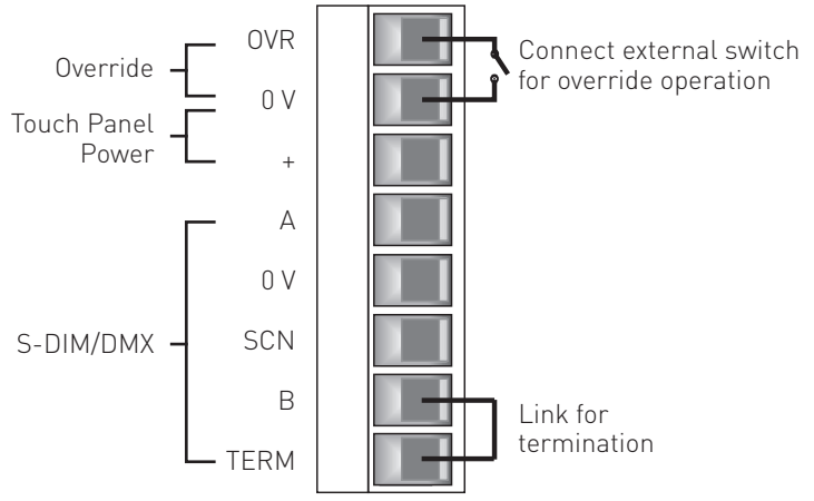
Touch Panel power, Override, and S-DIM/DMX connections
