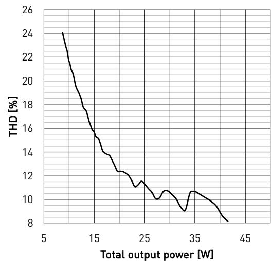
Current THD
