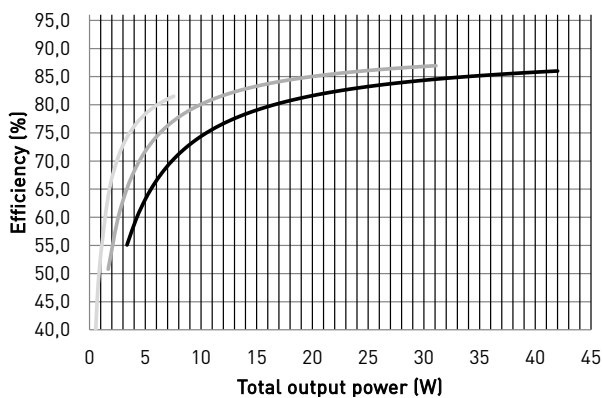
Typical efficiency
