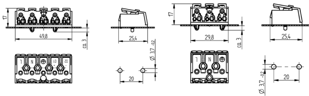
5 - pole connector for DA / CC drivers with LC-SRA-LOOP
