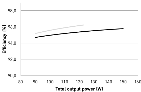
Typical efficiency
