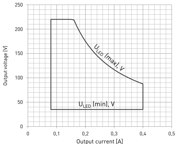
From 80 mA to 400 mA, full dimming range ( 1 % - 100 %) available in the whole area.
