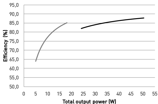
Typical efficiency
