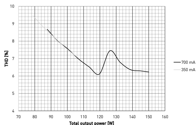
Current THD
